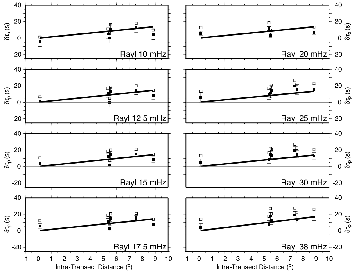
Figure 7. Same as Figure 6, but for fundamental-mode Rayleigh waves. See color version of this figure in the HTML.
