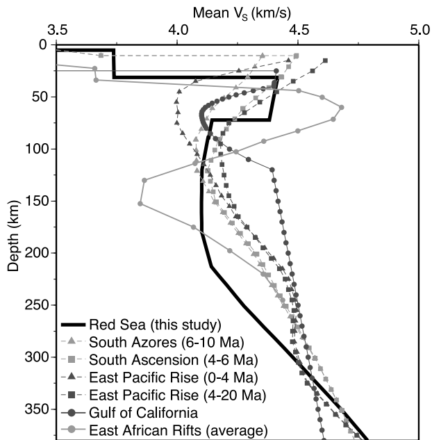
Figure 13. Comparison of the Red Sea upper-mantle shear velocity model (RS, bold black curve) developed in this study with velocity models from other continental rift and oceanic ridge environments. Light grey dashed curves: south Azores (6–10 Ma, triangles) and south Ascension (4–6 Ma, squares) sections of the mid-Atlantic ridge [Gaherty and Dunn, 2007]; Dark grey dashed curves: 0–4 Ma (triangles) and 4–20 Ma (squares) seafloor along the East Pacific Rise [Nishimura and Forsyth, 1989]; Dark grey circles: Gulf of California [Zhang et al., 2007]; Light grey circles: average velocities from the east and west branches of the East African Rift [Weeraratne et al., 2003]. See color version of this figure in the HTML.
