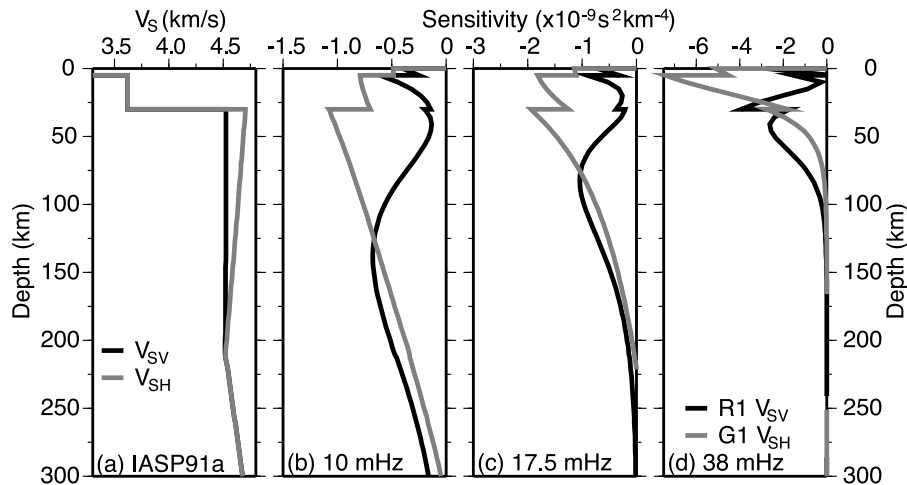
Figure 3. (a) Reference shear velocity model IASP91a, with V_{SH} shown in grey and V_{SV} shown in black. (b-d) Representative partial derivative kernels for fundamental-mode Rayleigh (black) and Love (grey) phase delays as a function of depth for three different frequencies. Reference model for all kernels is IASP91a; kernels shown all correspond to observations from event 00042112 at a station near the front-end of the Red Sea transect. The kernels are with respect to the most sensitive model parameter for each wave type, i.e., the Rayleigh wave kernel is for V_{SV} and the Love wave kernel is for V_{SH} . These kernels give a feel for the depth sensitivity of the phase-delay observations at different frequencies, with higher frequencies sensitive to shallower depths. Rayleigh waves sample deeper than Love waves at the same frequency. The kernels are negative because an increase in velocity leads to a decrease in phase delay [Gaherty et al. , 1996]. (b) Kernels for observations with center frequency of 10 mHz, which are sensitive well into the asthenosphere. (c) Kernels for 17.5 mHz observations, which are sensitive primarily to the upper asthenosphere. (d) Kernels for 38 mHz observations, which are most sensitive to crustal structure. See color version of this figure in the HTML.
