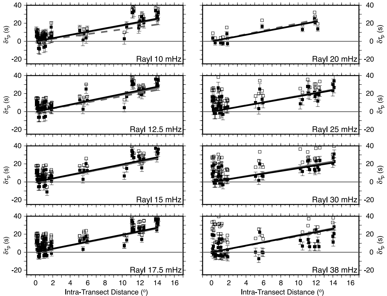
Figure 5. Same as Figure 4, but for fundamental-mode Rayleigh waves. Note the misfit to the lower frequencies when model RS is forced to return to IASP91a at 180 km depth (dashed grey lines). This indicates that the LVZ beneath the Red Sea transect must extend to depths greater than 180 km. See color version of this figure in the HTML.
