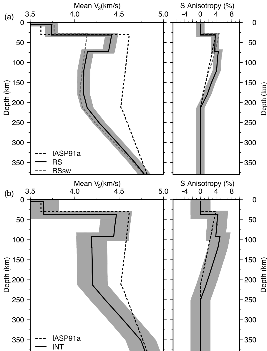
Figure 9. Radially anisotropic shear velocity models of upper-mantle structure beneath (a) the Red Sea transect (RS) and beneath (b) the interior transect (INT), derived from inversion of surface wave delays and receiver function constraints. The grey shaded areas show the associated uncertainties reported in the text; however, quantification of the base of the LVZ also suggests that resolution below \sim 210 km is poor. Also shown in (a) is model RSsw (grey dashed curves), which is the preferred subarray model for the Red Sea transect obtained by only using the surface wave delay times (without including the receiver function S-P constraints in the inversion). In both (a) and (b), the left panel displays mean shear velocity ( V_S = (V_{SH} + V_{SV})/2 ), while the right panel displays shear anisotropy ( \Delta V_S = (V_{SH} - V_{SV})/V_S in percent). Reference model IASP91a is shown by the black dashed curves. See color version of this figure in the HTML.
