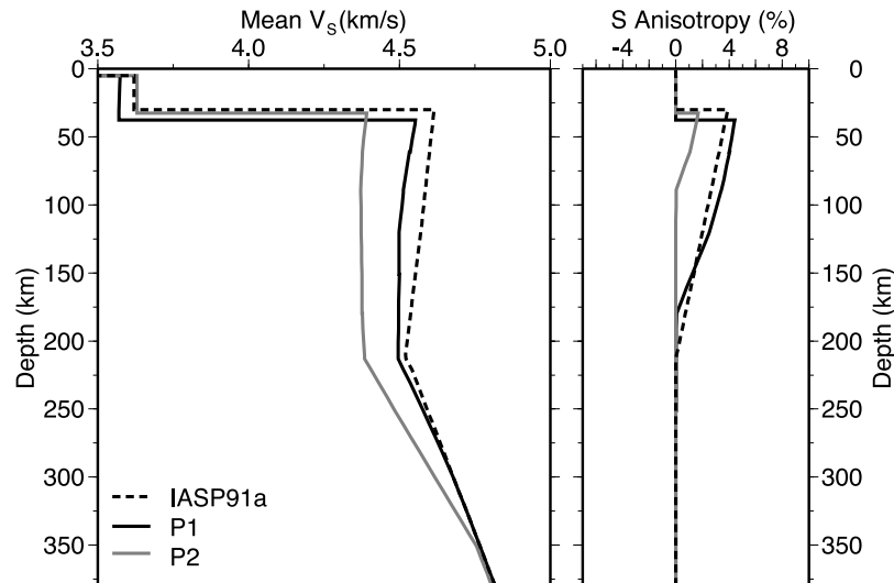
Figure 8. Radially anisotropic shear velocity structure of path models P1 (solid black curves) and P2 (solid grey curves). Also shown is the reference model IASP91a (black dashed curves). Left panel displays mean shear velocity ( V_S = (V_{SH} + V_{SV})/2 ), while right panel displays shear anisotropy ( \Delta V_S = (V_{SH} - V_{SV})/V_S in percent). See color version of this figure in the HTML.
